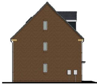
L.H. SIDE ELEVATION.
